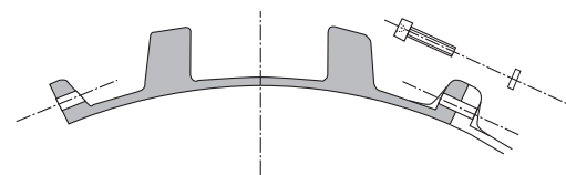
Sectional drawing of RGV segment
