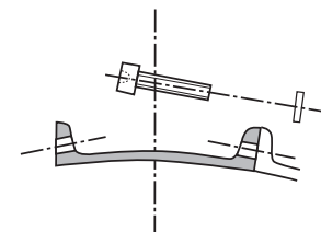
Sectional drawing of MA 2 segment
