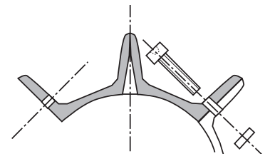
Sectional drawing of AZ/AC 1 segment
