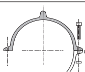
Sectional drawing PA/PE 0.75 to PA/PE 4, ring with 4 skids total
