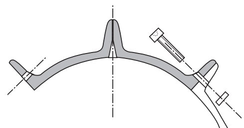
Sectional drawing of AZ/AC 2 segment
