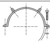
Sectional drawing PA/PE 6 to PA/PE 12, ring with 6 skids total
